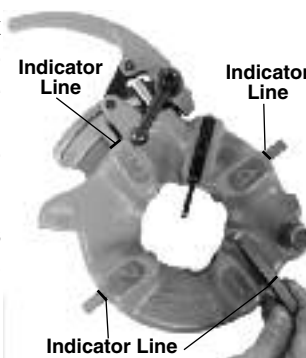
Figure 12 – Inserting Dies
