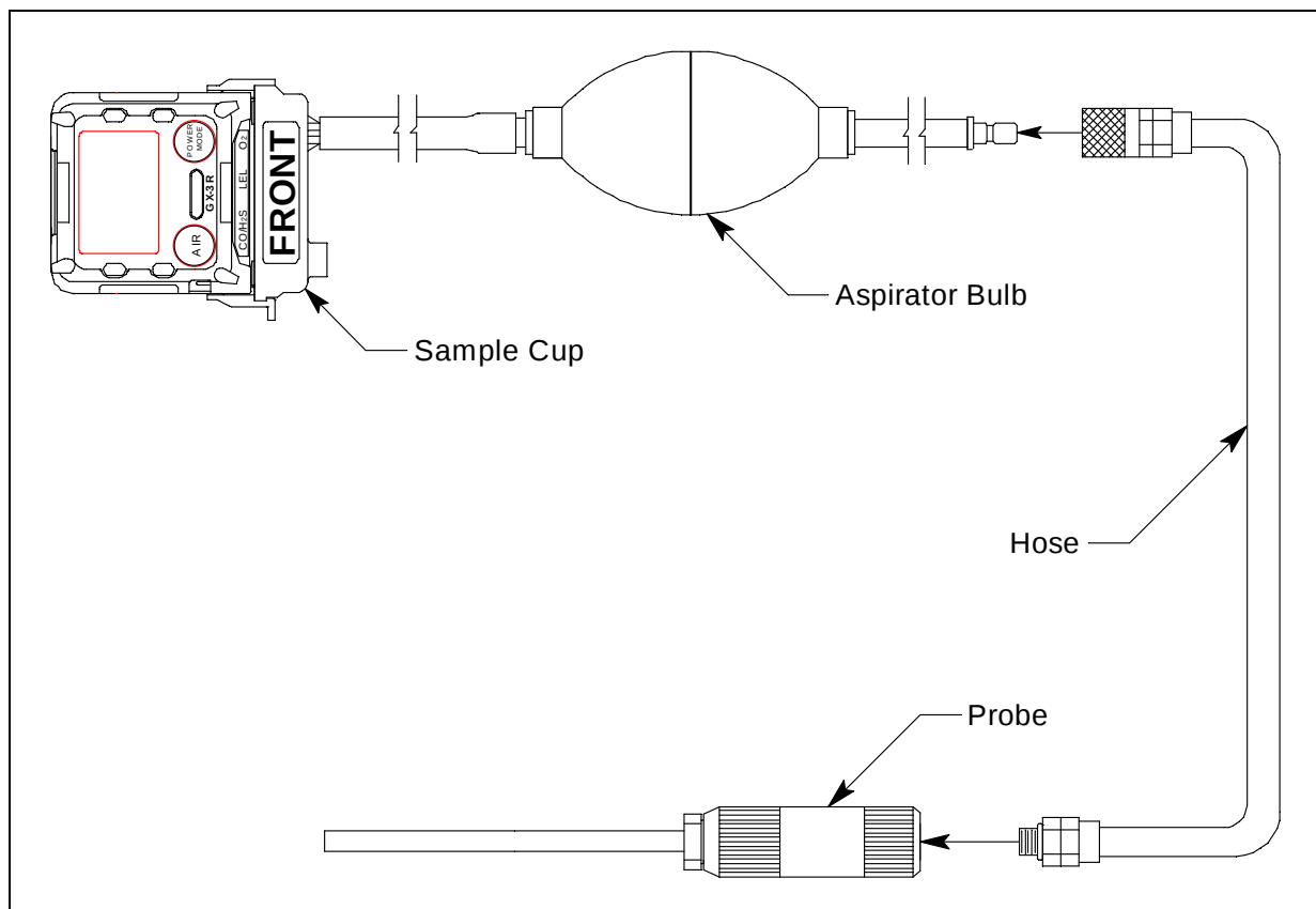
Figure 6: GX-3R Aspirator Adapter
