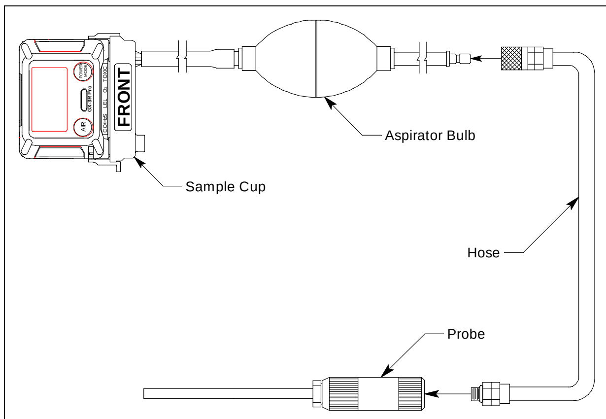
Figure 6: GX-3R Pro Aspirator Adapter
