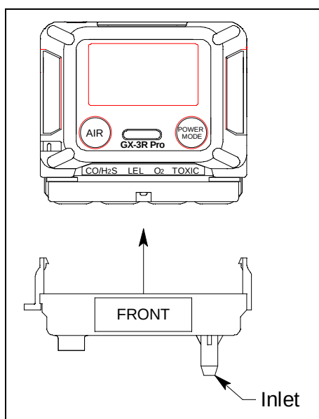
Figure 28: Calibration Cup Installation
