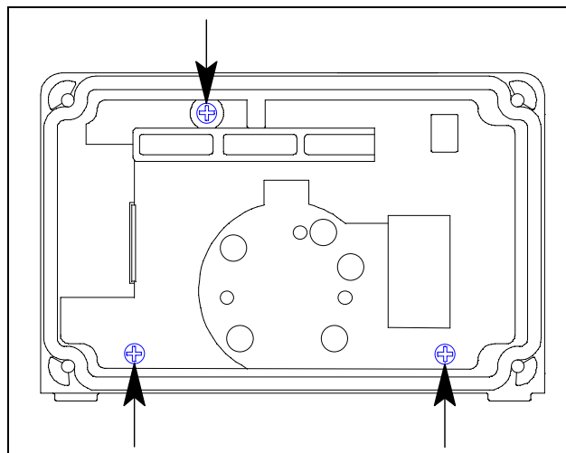
Figure 20: Removing Battery Board Screws
