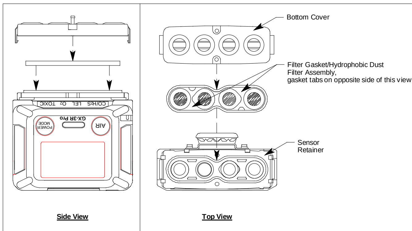
Figure 17: Replacing the Hydrophobic Dust Filter
