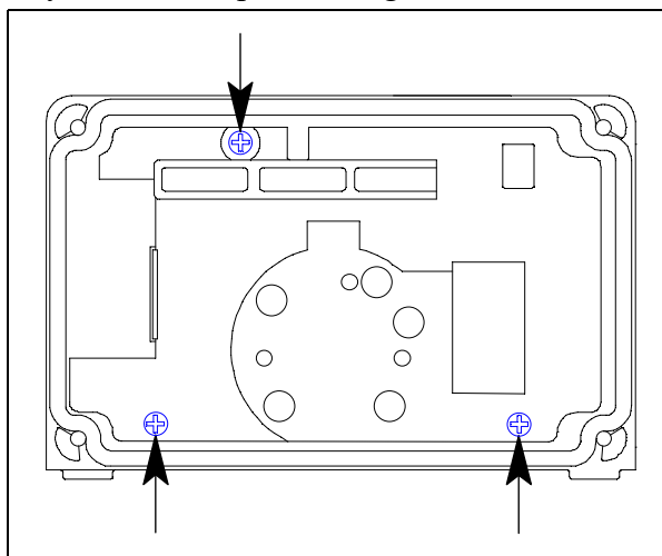
Figure 23: Reinstalling Battery Board Screws
