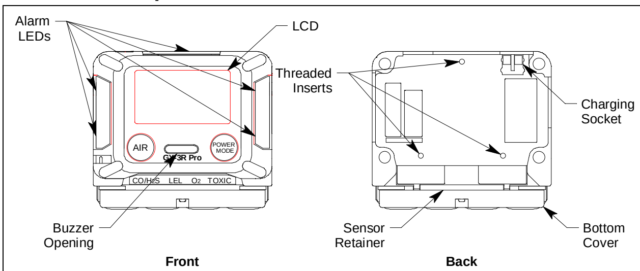
Figure 1: Component Location
