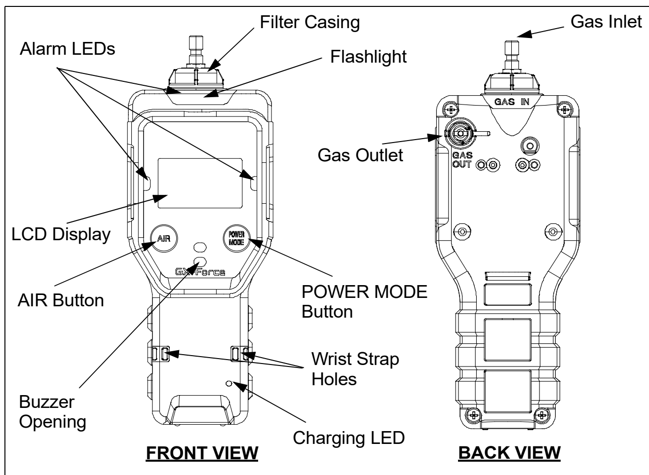
Figure 1: Component Location
