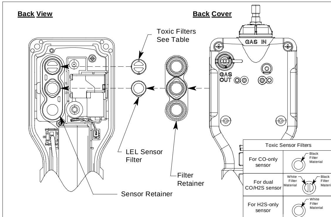
Figure 8: Replacing the Sensor Filters
