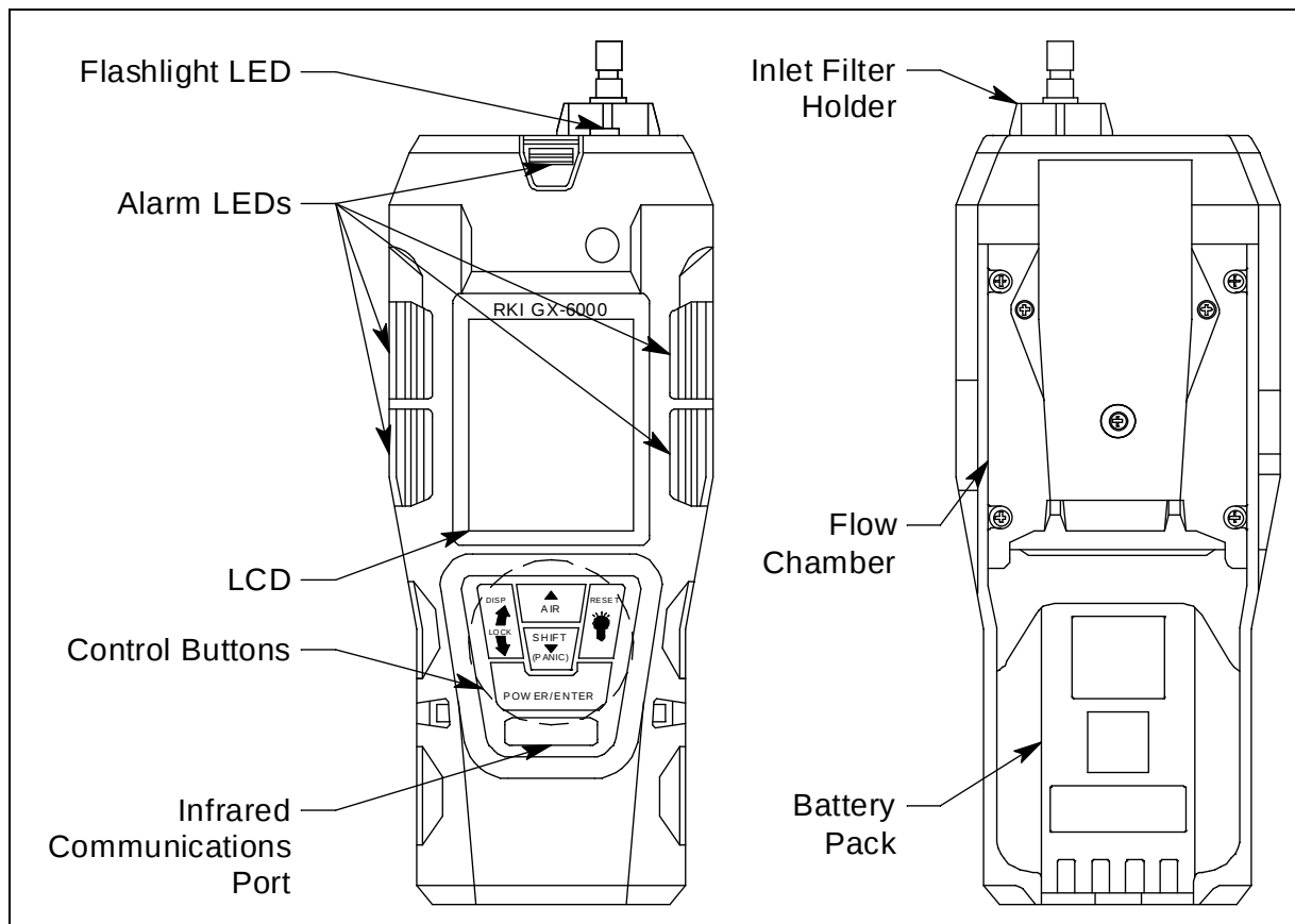
Figure 1: Component Location
