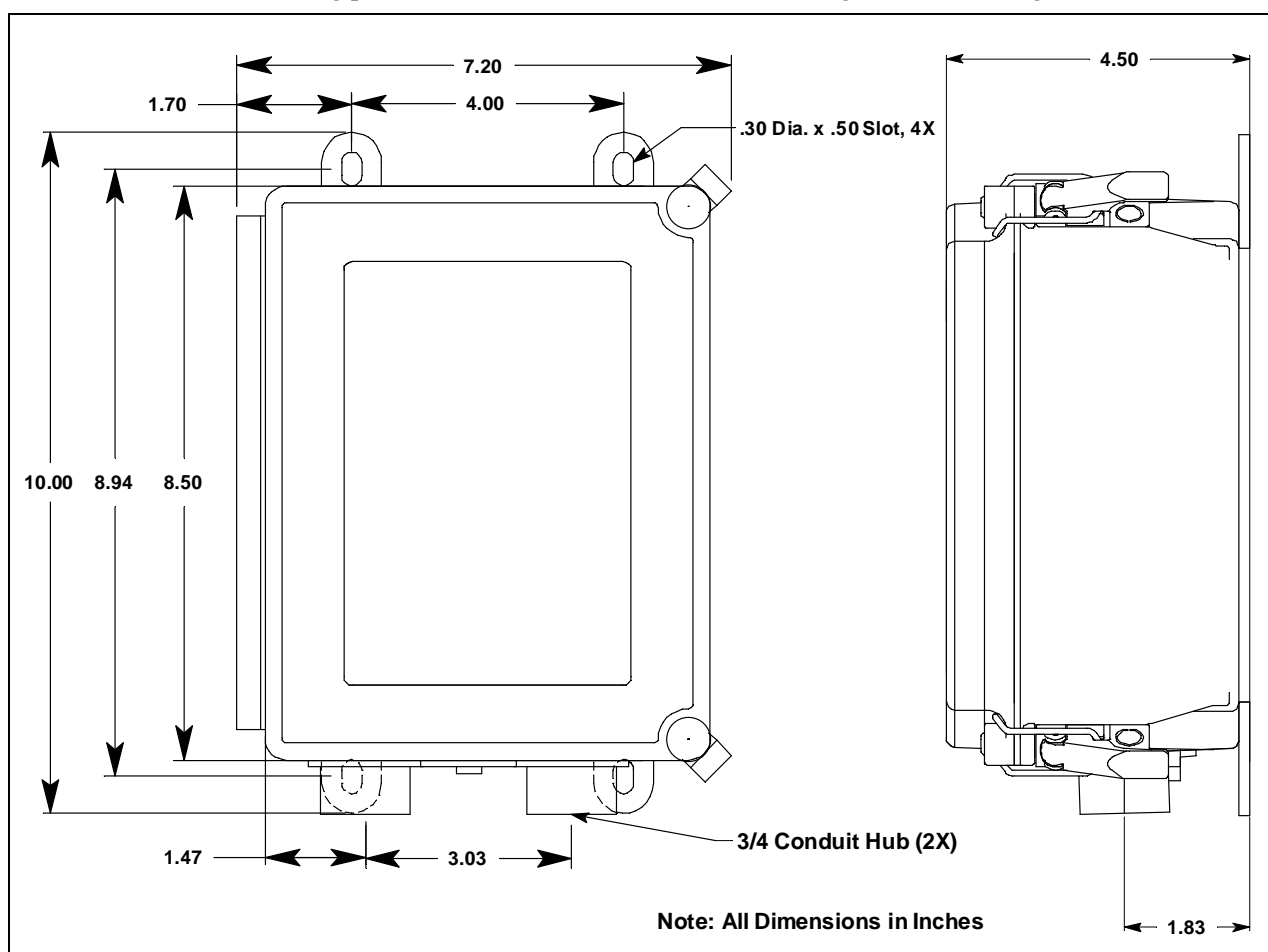
Figure 6: Beacon 110 Dimensions
