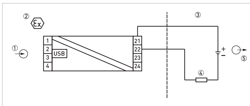
Figure 4-4: Connection diagram
