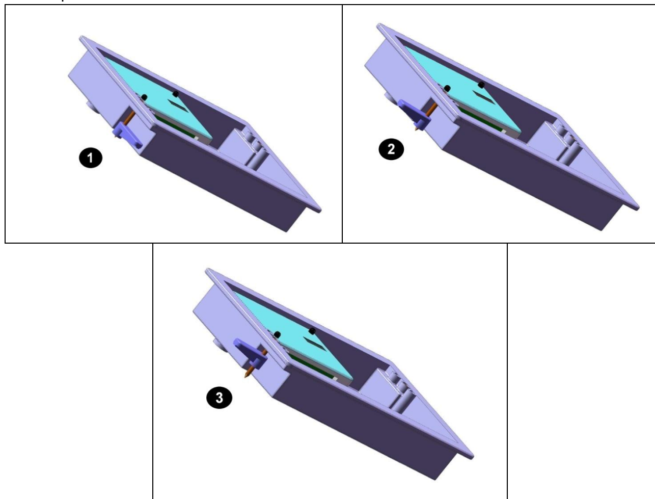
Figure 4: Enclosure installation
