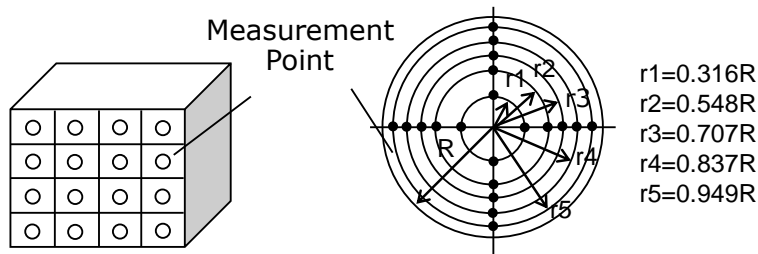
Rectangular Duct
