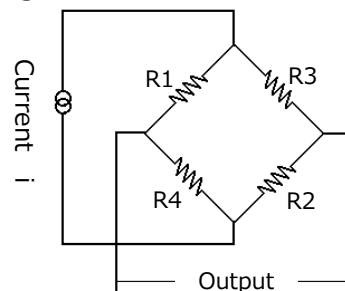
Pic.3 Detecting Circuit
