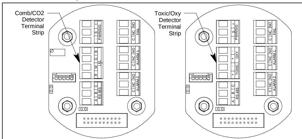
Figure 11: Detector Terminal Strip
