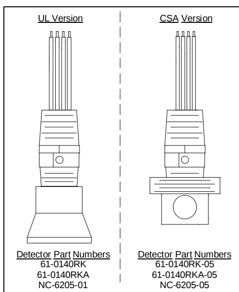
Figure 2: Catalytic Sensors
