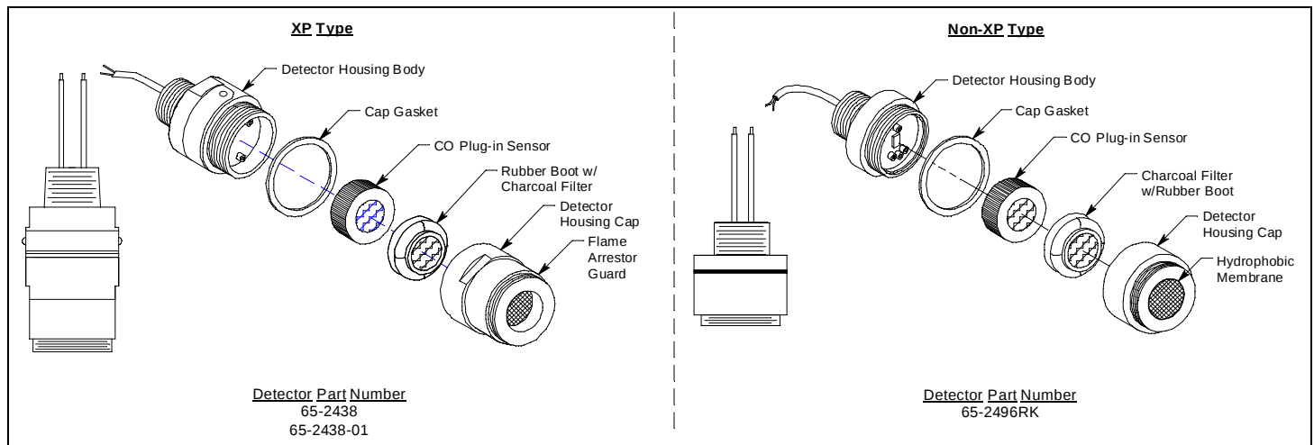
Figure 6: CO Detectors
