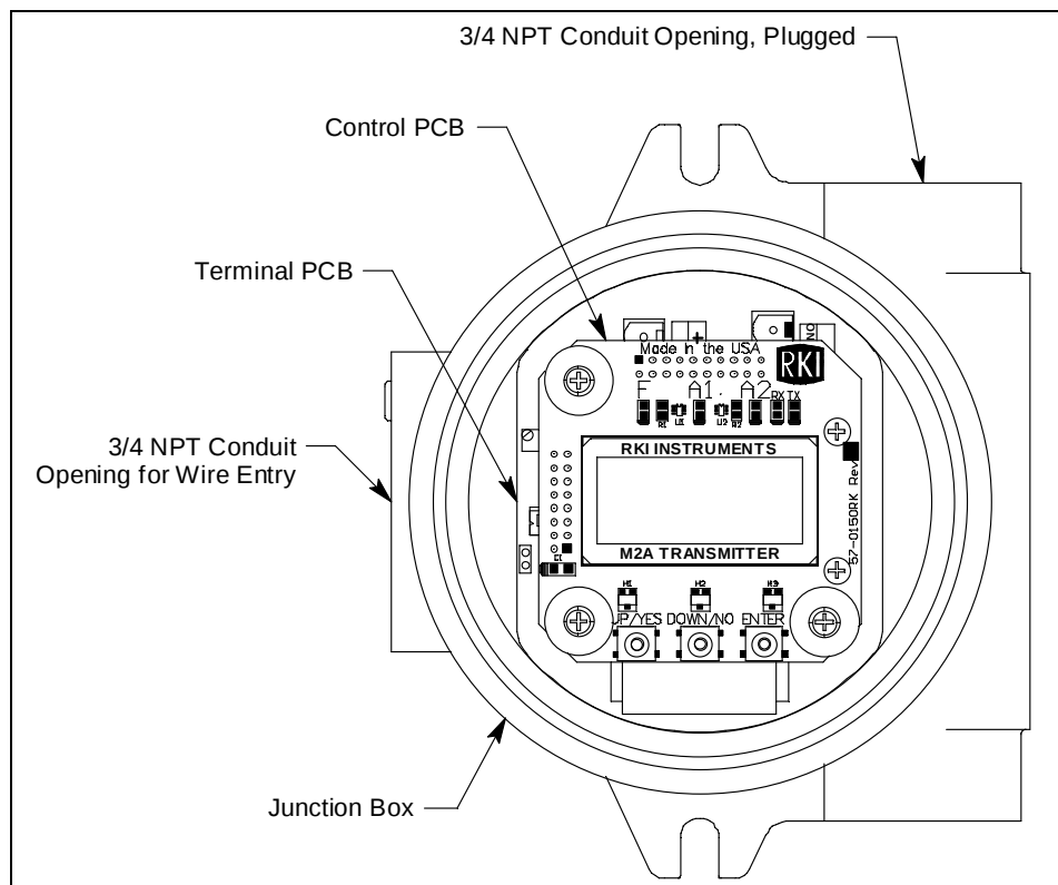
Figure 9: M2A Internal Components
