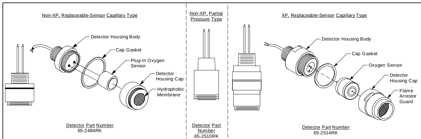
Figure 4: Oxygen Detectors
