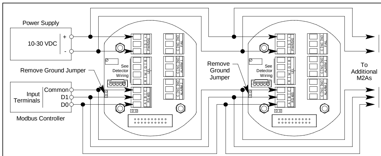
Figure 32: Recommended Modbus Wiring
