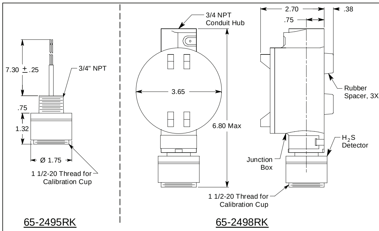
Figure 3: Outline & Mounting Dimensions, 65-2495RK & 65-2498RK
