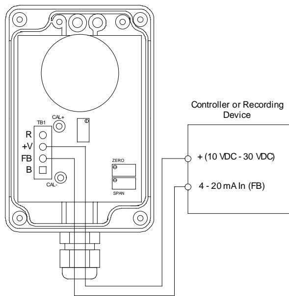
Figure 3: Wiring the CO Transmitter to a Controller
