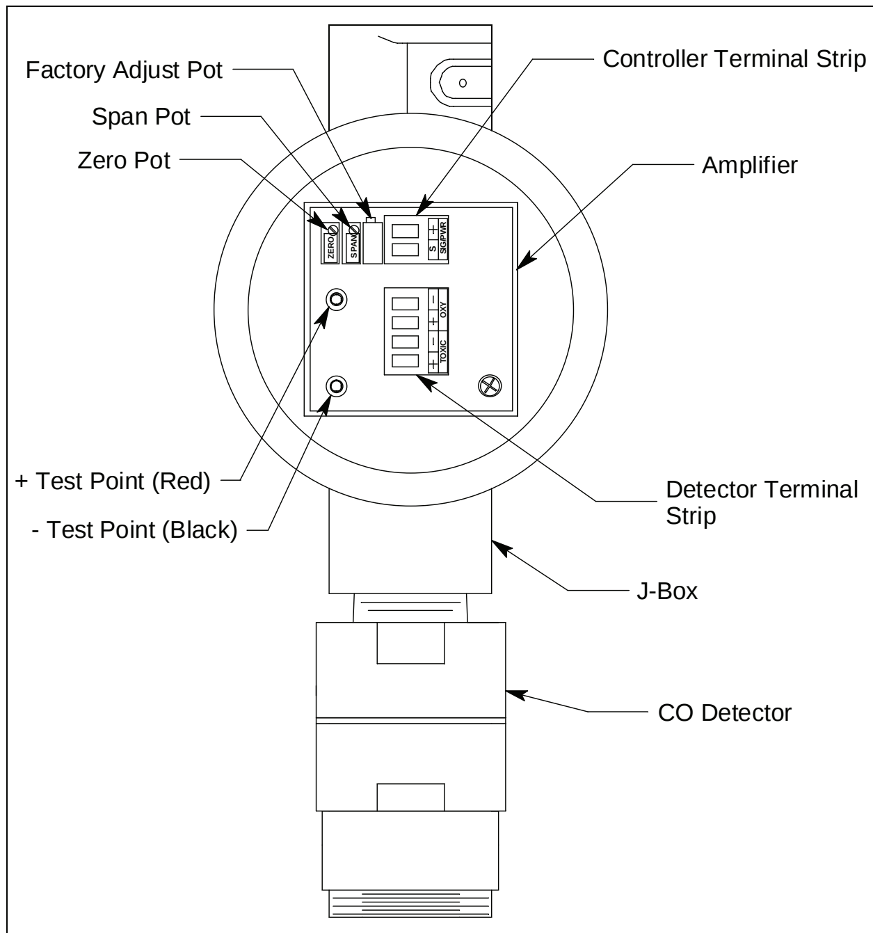
Figure 1: CO Transmitter Component Location
