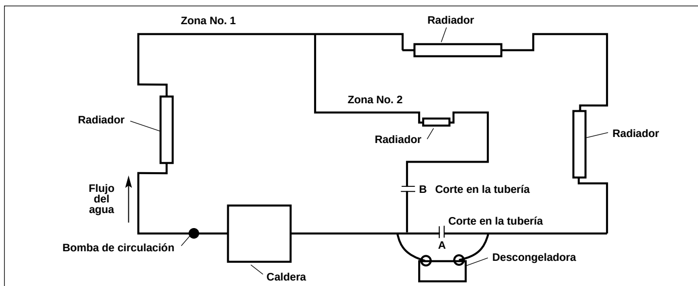
Figura 7 – Red multizona
