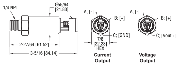
Fig. F: Packard Connection
