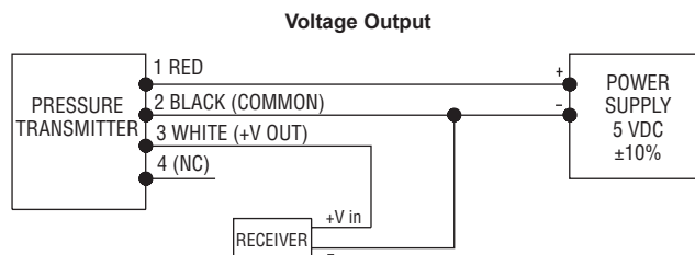
Fig. K: Voltage output connection
