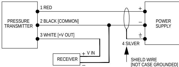
Figure E: Voltage output connection
