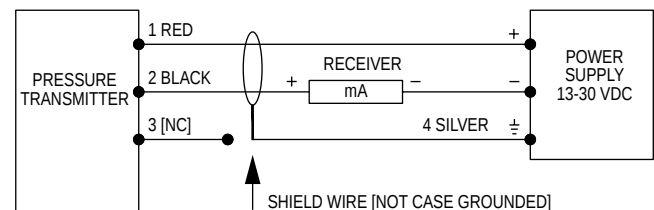
Figure A: Current output connection
