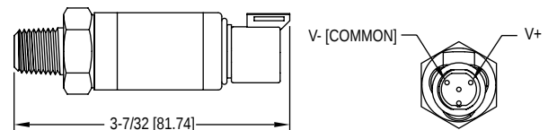
Figure P: Deutsche connection, 4-20 mA output
