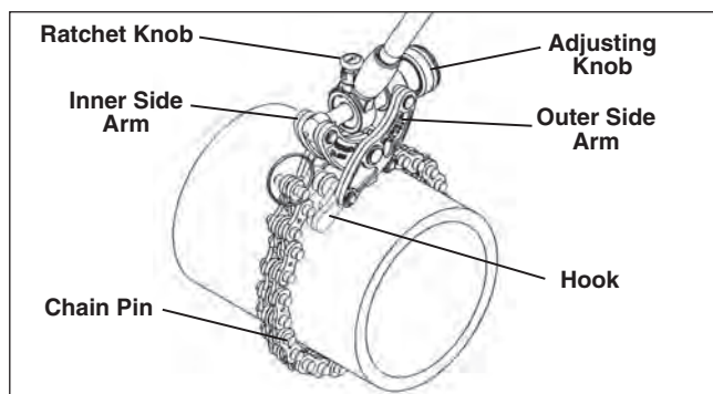
Figure 5 – 206/246 Soil Pipe Cutter
