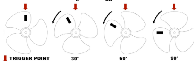
Figure 9 Triggered Phase
