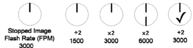
Figure 3 Object rotating at 3000 RPM
