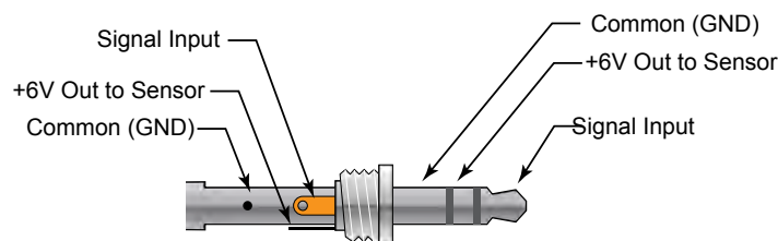
Figure 2 Input Connector Detail (Stereo plug)
