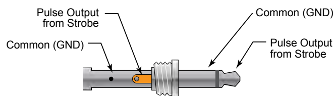
Figure 3 Output Connector Detail (Mono plug)
