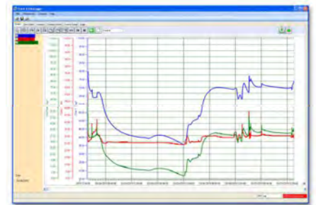
Track-It Software
