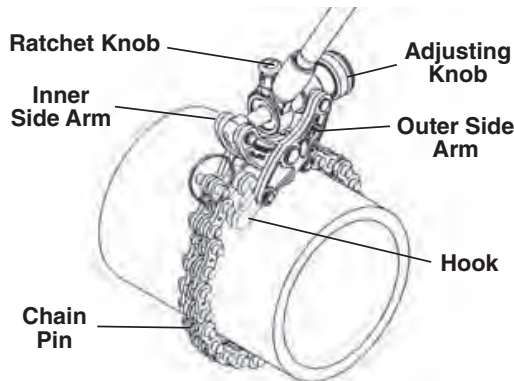
Figure 5 – 206/246 Soil Pipe Cutter
