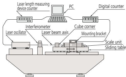
[Figure 1] Linear scale accuracy inspection device, overview
