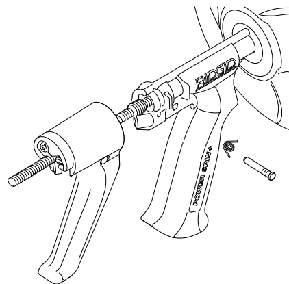
Figure 10 – Trigger Assembly
