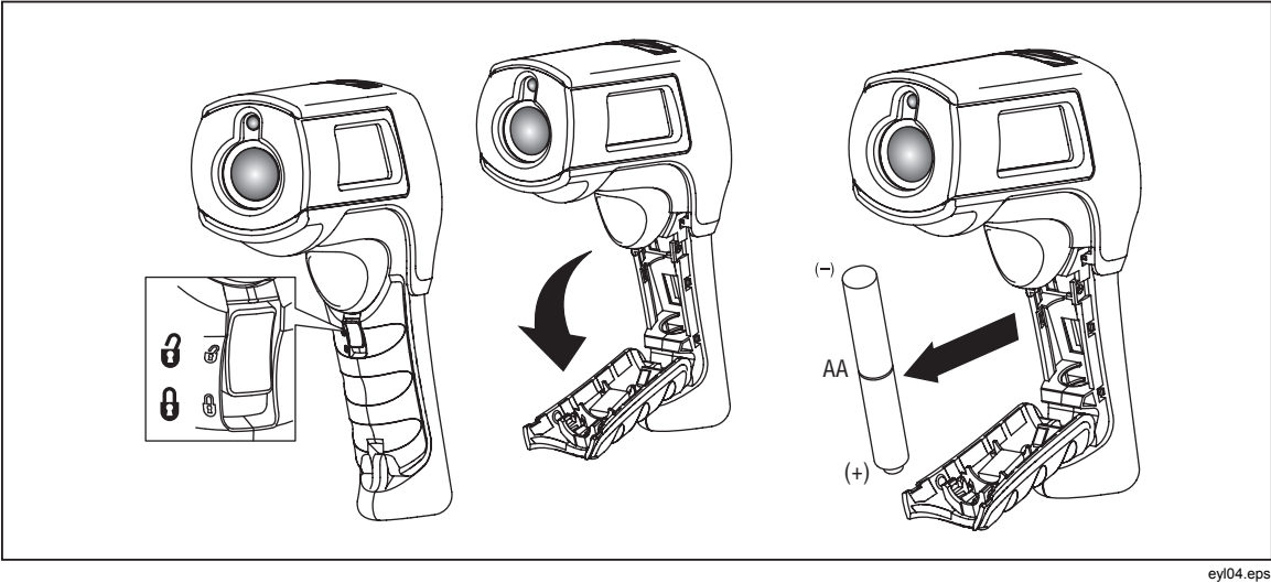
Figure 10. Battery Replacement
