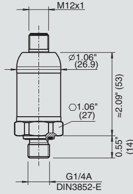
with M12 x 1 circular connector (4-pin, metallic)
