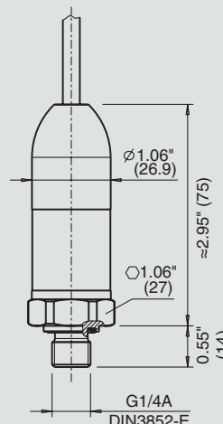
with cable outlet IP 68, FEP, IP 6K9K
