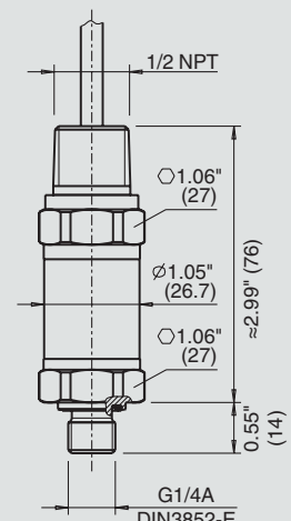
with cable outlet 1/2 NPT conduit
