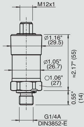
with circular connector M12 x 1 (4-pin)
