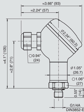
connection head with terminal block
