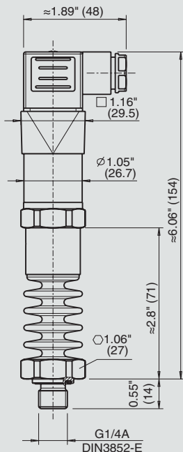
with angular connector DIN 175301-803 A and cooling element
