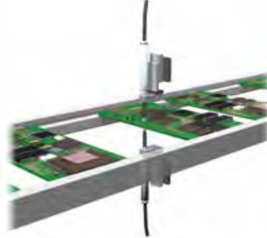
2 PCB thickness measurement
