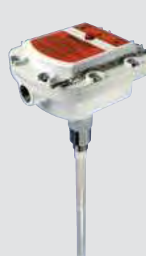
PRO AUTO-CAL Auto-Calibrating Capacitance Probe
