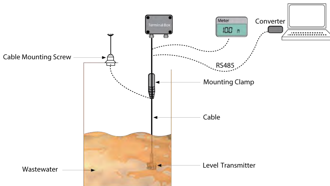
Fig.2. Mounting the transmitter
