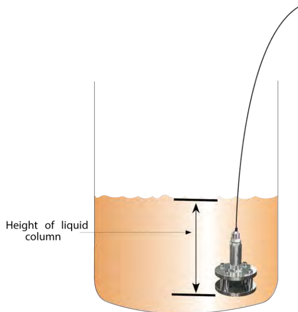
Fig.1. Measuring Principle
