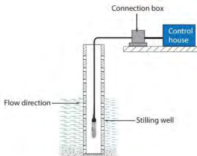
Fig.5. Installation in flowing liquid
