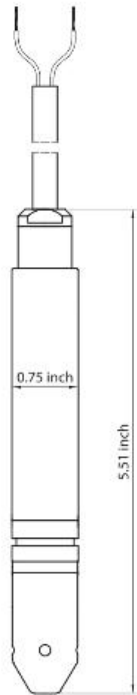
Fig.3 Dimension Drawing
