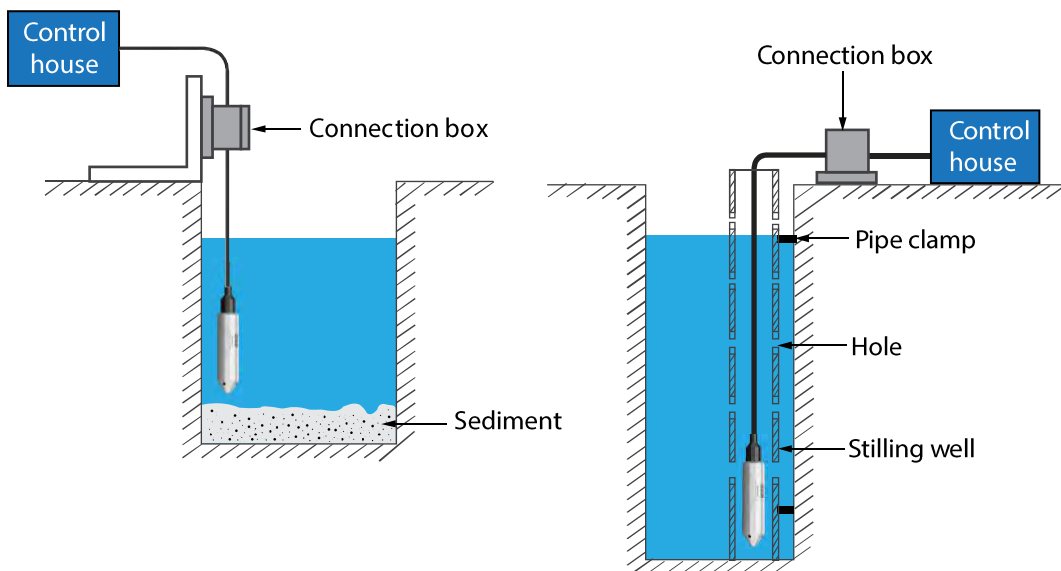
Fig.4. Installation in static liquid
