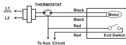
TAC Erie Wire Leads
