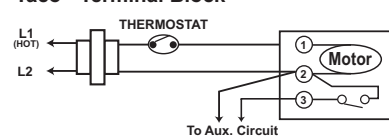
Taco - Terminal Block
