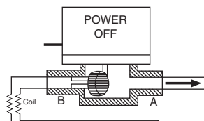
Figure-6a 2-Way Valve With Normally Closed Actuator.
