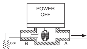
Figure-6b 2-Way Valve With Normally Open Actuator.
