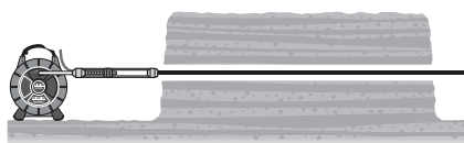
Figure 11 – Connect Air Hose To The CROSSCHEK Inspection System
