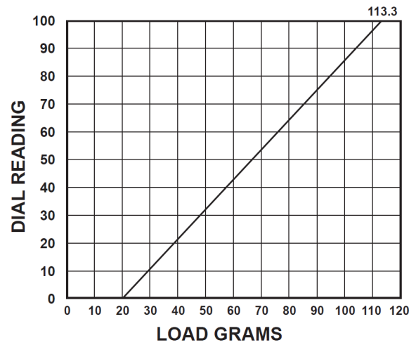
Force curve for Model 411 (ASTM D2240 Type OO)
