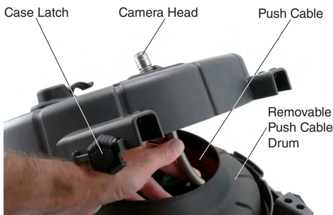
Figure 2 – Inside Case
