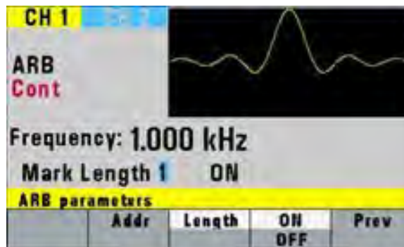
Figure 3.5 - Marker Menu
