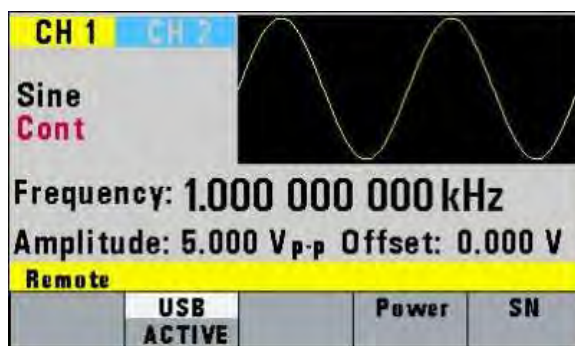
Figure 3.22 - Utility Menu
