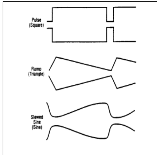
Figure 4. Effects of Symmetry Variation.
