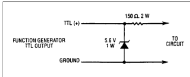
Figure 5. Circuit for Protection of TTL Output.
