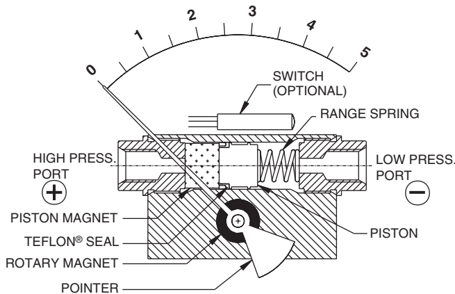
Model 1130 Piston
