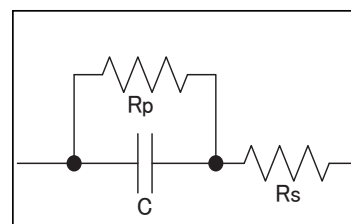
Equivalent circuit of capacitors
