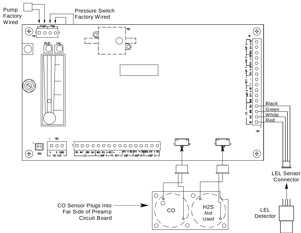
Figure 6: Internal (Factory) Wiring, Sample Draw Detector
