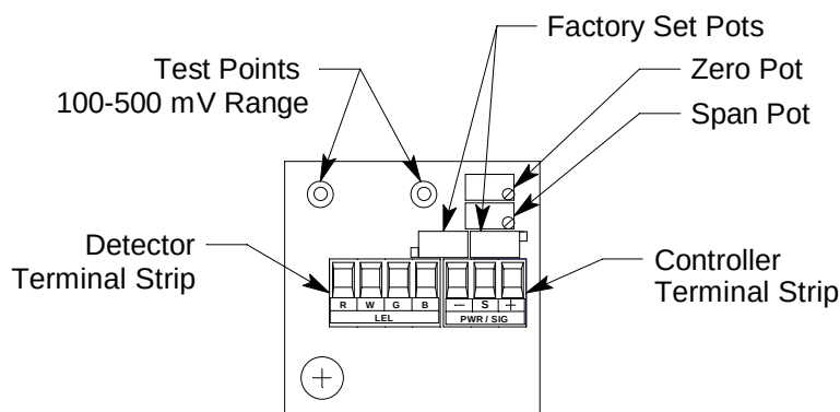
Figure 3: Amplifier Component Location
