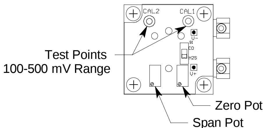
Figure 3: H 2 S Amplifier Component Location
