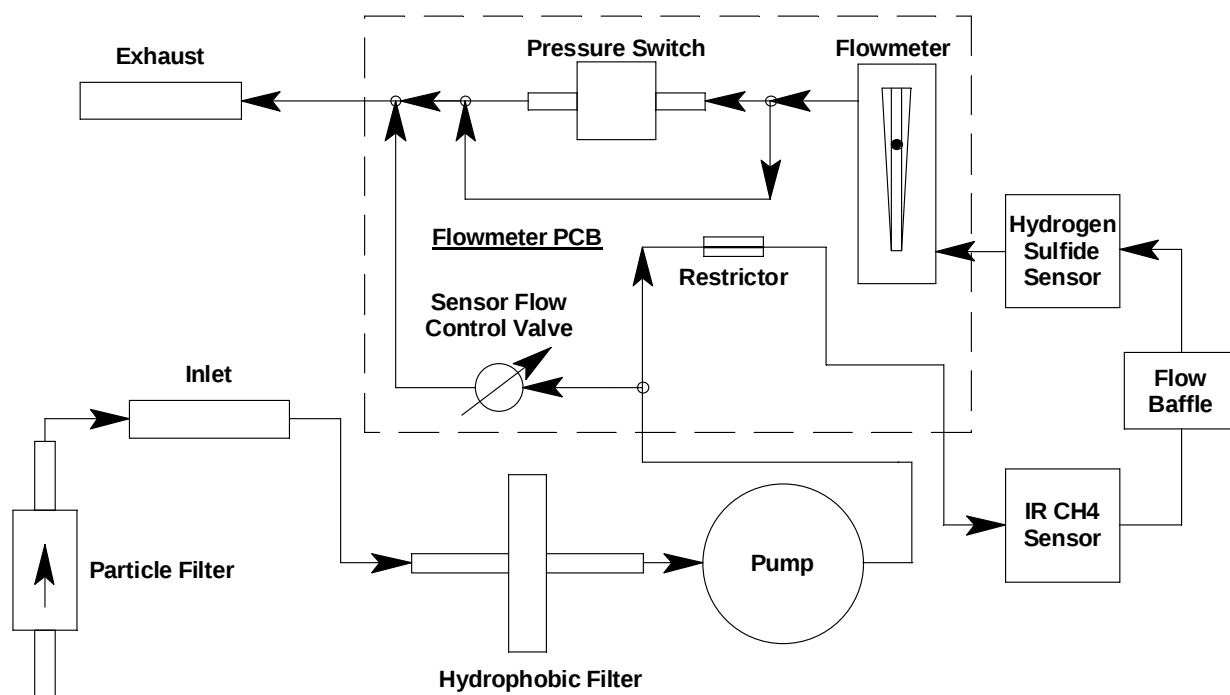
Figure 2: Methane/Hydrogen Sulfide Sample-Draw Detector Flow Diagram
