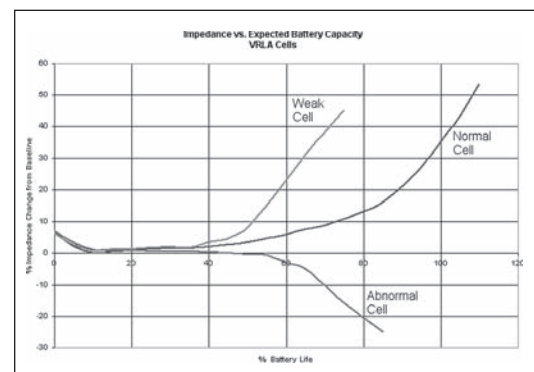
Figure 4. Impedance increases with battery age (and weakness)
