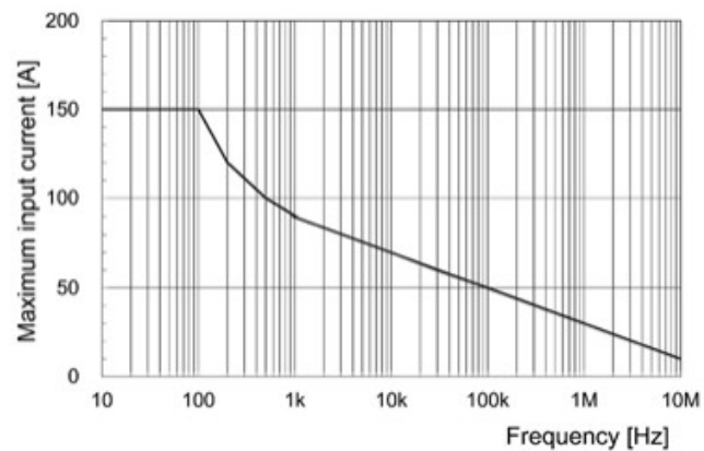
Fig.3 Derating according to frequency(3274)
