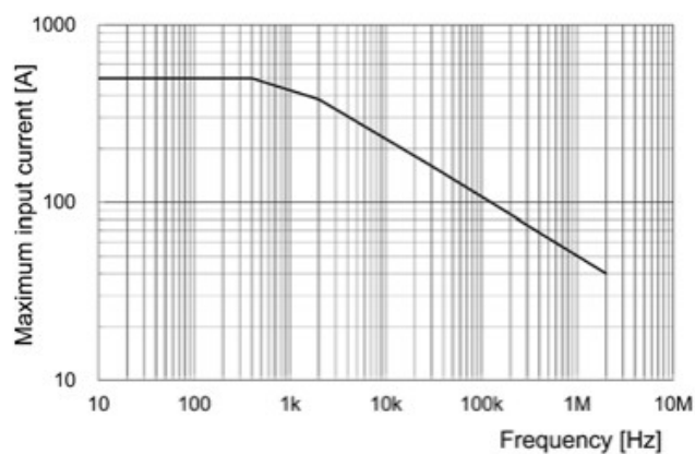
Fig.4 Derating according to frequency(3275)
