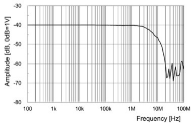
Fig.2 Frequency characteristics (Typical) (3275)
