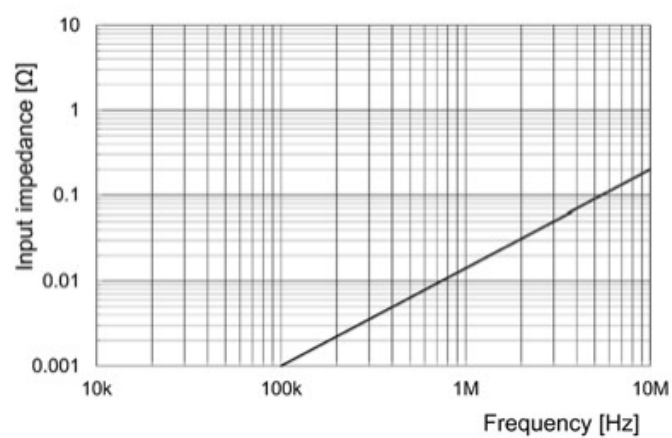
Fig.5 Input impedance (Typical) (3274)
