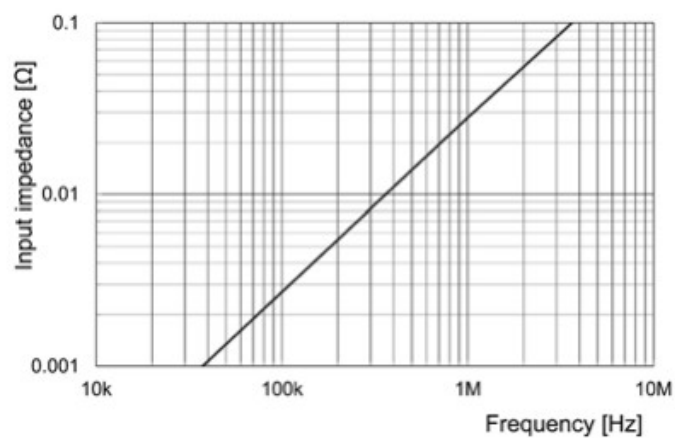
Fig.6 Input impedance (Typical) (3275)
