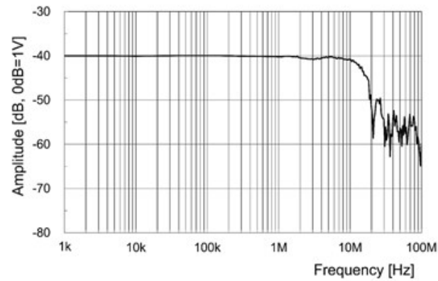
Fig.1 Frequency characteristics (Typical) (3274)
