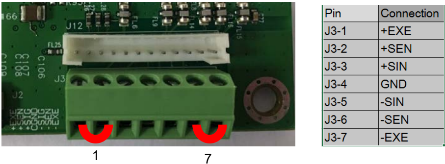
Figure 2-4 Jumper Connections
