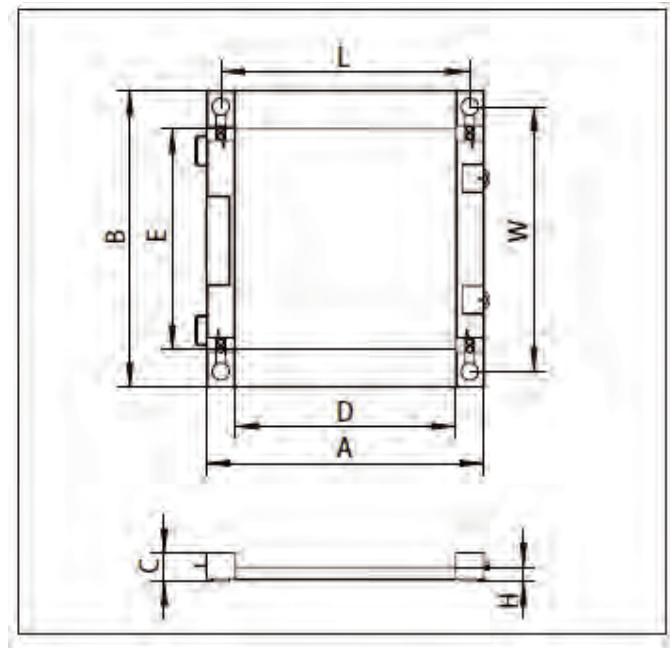
Figure 2. Drum Scale Dimensions
