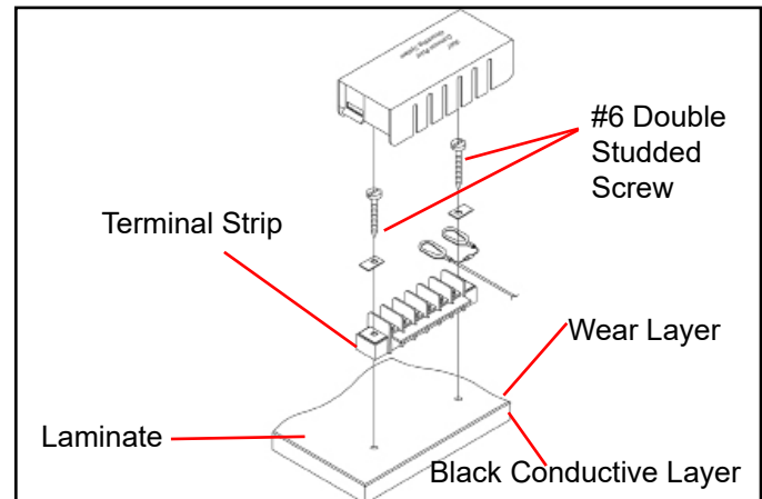
Figure 3. Installing the 3047 Common Point Grounding System (top).
