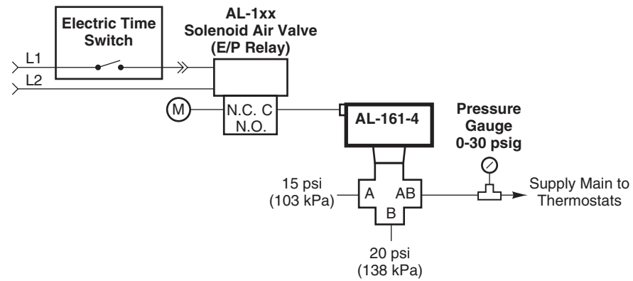
Figure 1 Typical Application.
