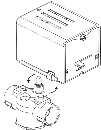
VT/VS Series with High Close-Off Actuator
